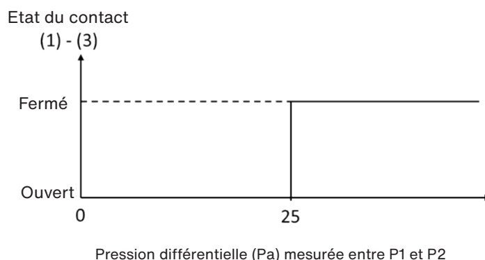
Pressostat DEP S – DEP R ECO - DIVA
