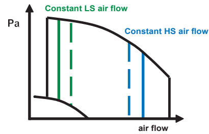
EXAECO® + MAC2 EC® operation
