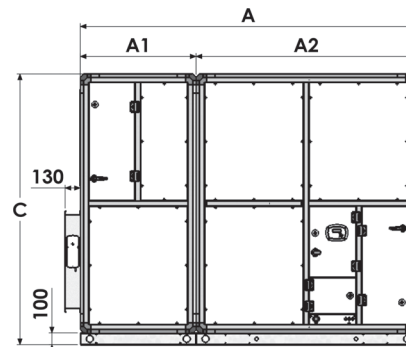
SIDE VIEW EXAECO®
