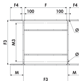
TOP VIEW OF EXAECO® FRAME AND FEET MODULES ELITE ®
