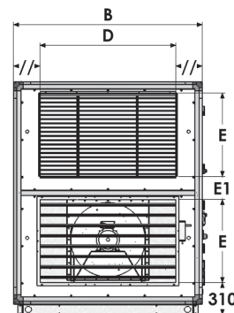
SIDE VIEW EXAECO®
