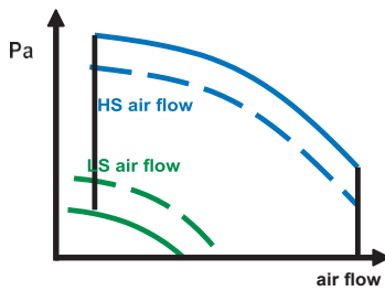
EXAECO® operation
