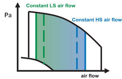
EXAECO® + QUATTRO EC® operation
